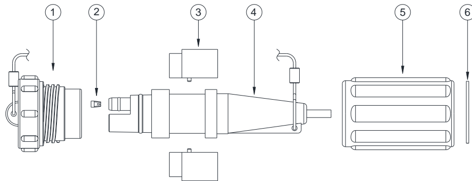
HGS 5515M Marine SF Conn.
