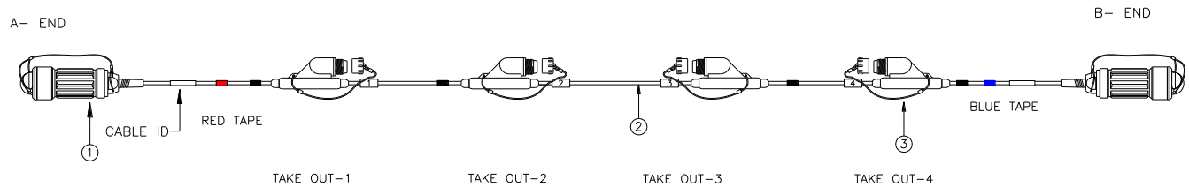
G3i LAND CABLE with 4 Channel
