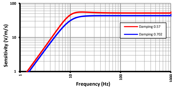
Response curve
