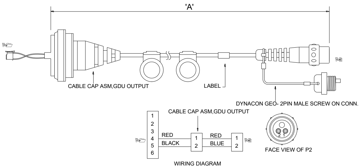
Cable Assy., GDU to Dynacon
