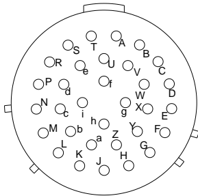
FACE VIEW
