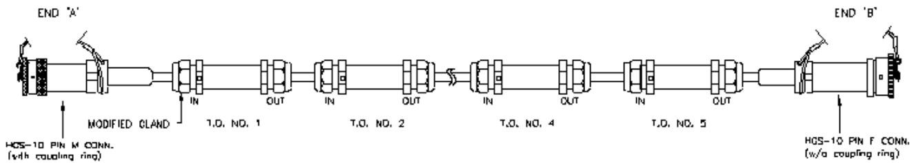
Saris Resistivity imaging cable with 5 take outs
