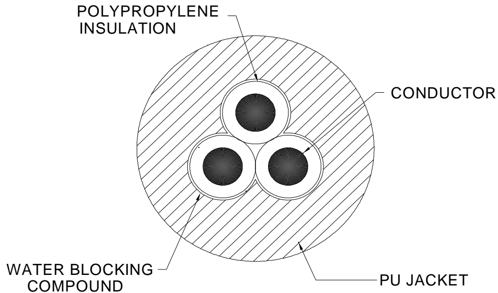
GEOPHONE LEADER CABLE (3 CORE)
