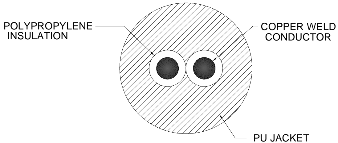
GEOPHONE LEADER CABLE(2 CORE)
